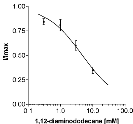
FIGURE 2 Dose-response curve of the effect of 1,12-diaminododecane on BK single-channel current amplitudes. Holding potential 0 mV, n = 4 .
